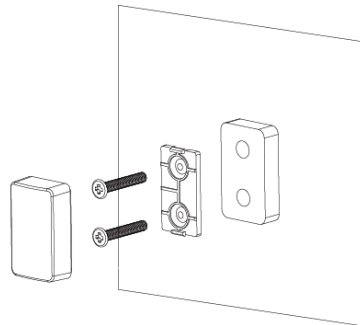
Screw Mount with Spacer
